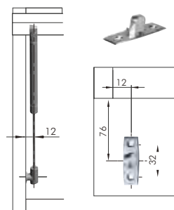
BRACKET: SCREW FIXING
