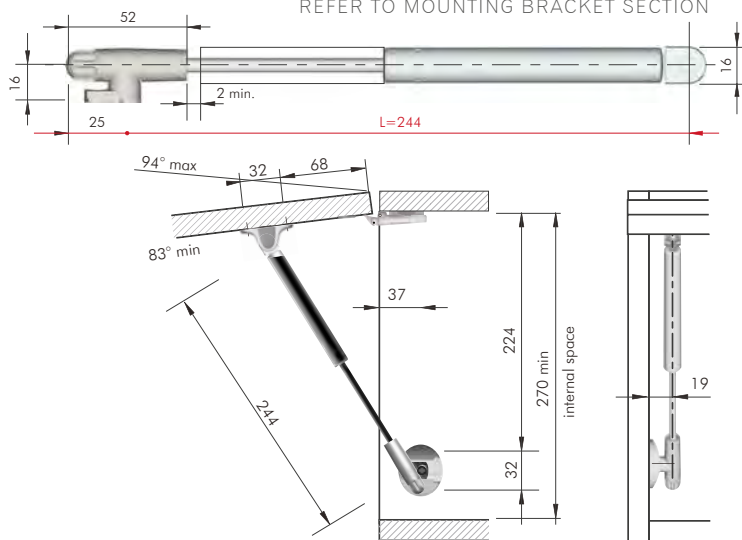
DRILLING DETAIL
