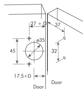
Drilling detail for the Pie Cut hinge
