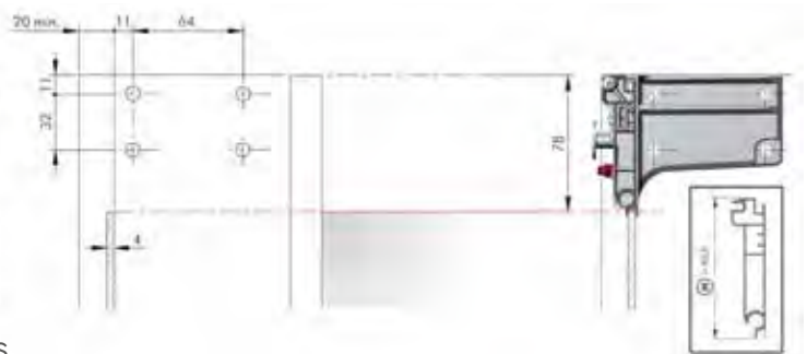
DRILLING PLAN WITH BACK PANEL WOOD THICKNESS 4MM AND H. 80,5MM ALUMINIUM BAR
