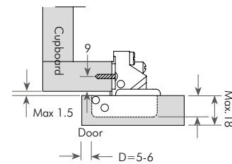
Drilling detail for face frame
