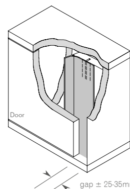
INTERNAL CORNER 901 013
