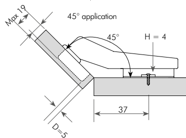
Drilling detail for 45° hinge
