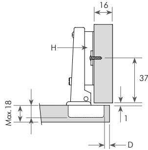
Drilling detail for the 110° Full Overlay & Half Overlay
