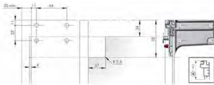
DRILLING PLAN WITH BACK PANEL WOOD THICKNESS 4MM AND H. 40,2MM ALUMINIUM BAR
