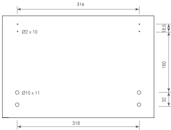
Internal Cabinet Detail
