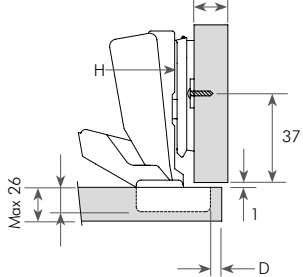
180° Full Overlay
