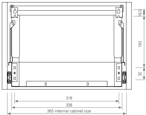
Internal Cabinet Detail
