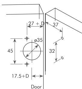
Drilling detail for the 180° Full Overlay & Half Overlay
