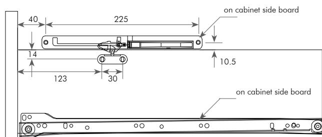
Installation for Drawer Slide
