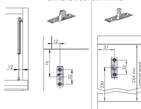
BRACKET: SCREW FIXING
