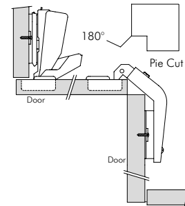
Face Frame application
