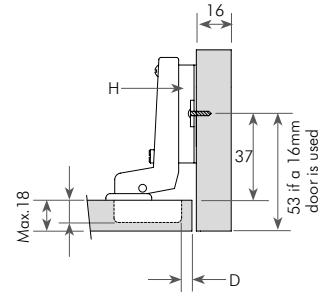
110° Inset application
