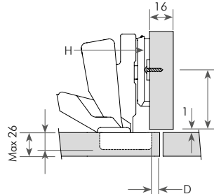
180° Half Overlay application
