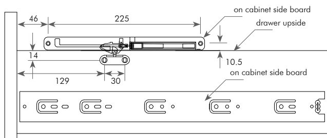
Installation for Ball Bearing slide
