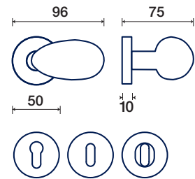
rosette - bocchette 10 mm rosettes - escutcheon
