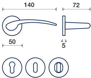
rosette - bocchette 5 mm rosettes - escutcheon
