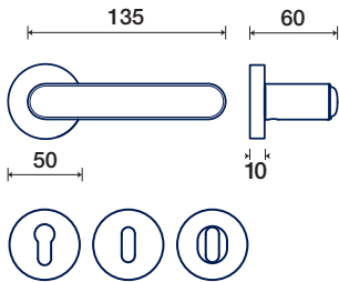
rosette - bocchette 10 mm rosettes - escutcheon
