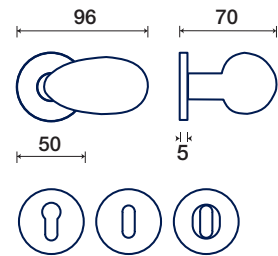
rosette - bocchette 5 mm rosettes - escutcheon
