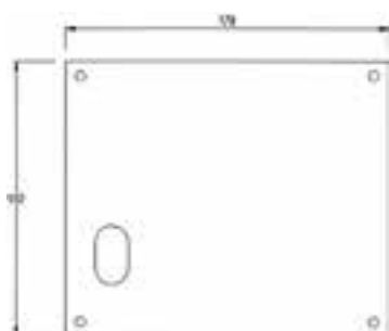
UNION 178x152mm AL5067-06AS Blank AL5067L/R-05AS Euro AL5067L/R-13AS Oval AL5067L/R-24AS Keyhole
