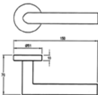
Sandpiper Lever Handle
