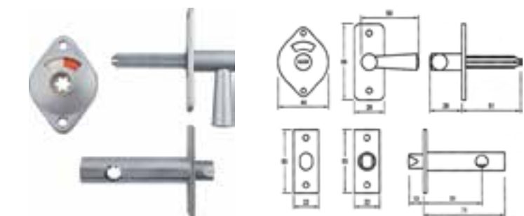
WC Indicator Bolt
