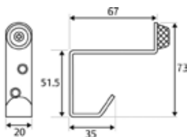
Hat and Coat Hook with Buffer UNION SS8025SS
