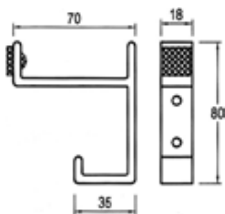
Coat Hook Rubber Tipped UNION AL8722AS
